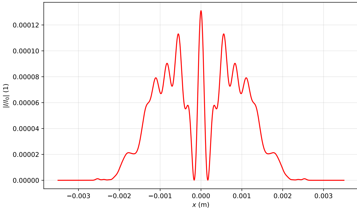
Intensity profile I(x, y = 0, z = 1.274)/I_0 , P_{in}=8.0P_{cr} , artificial time
